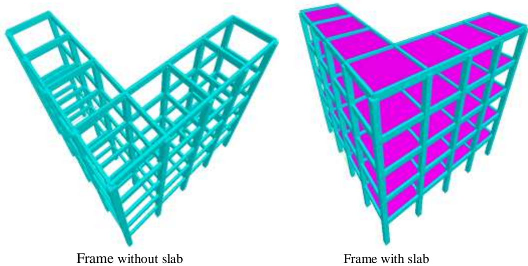
Fig 1 Isometric view of L shaped building
