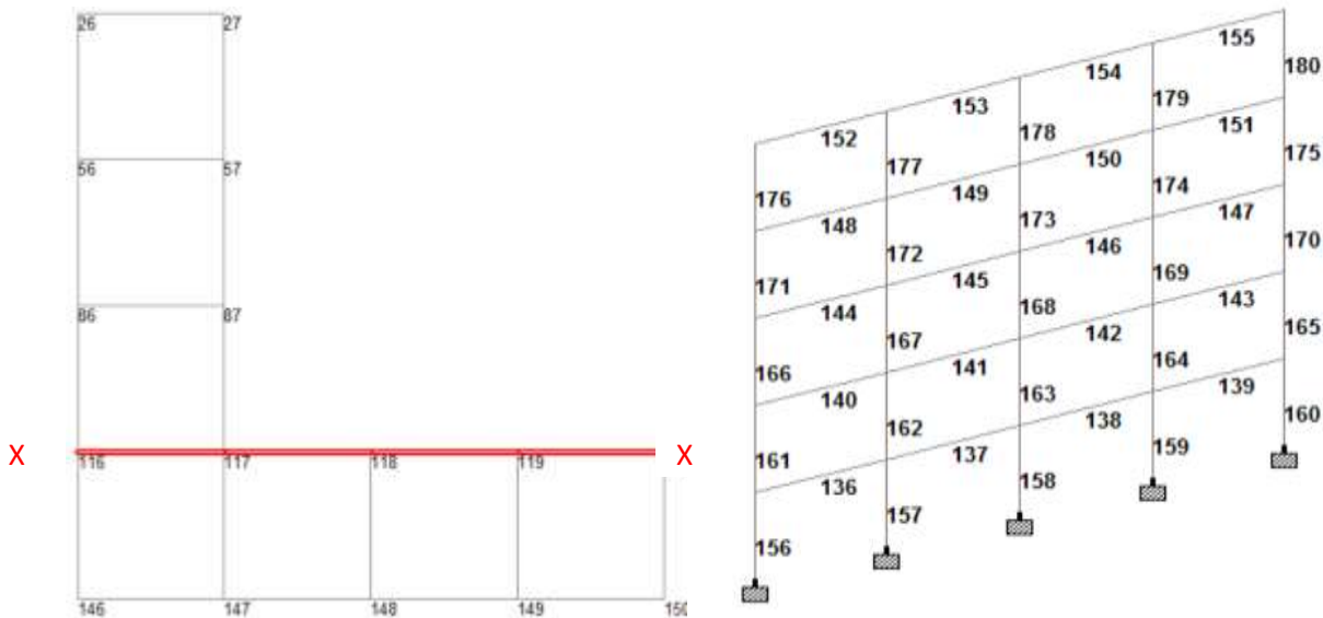
Fig 5 Beams and column numbering at section X-X
